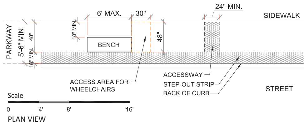
Diagram 2. Required dimensions for installing a bench in the parkway
