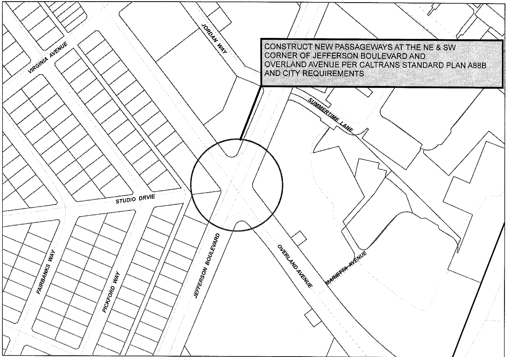
PEDESTRIAN ISLAND MODIFICATION PROJECT, P- 915 (OVERLAND AVENUE AND JEFFERSON BOULEVARD)
