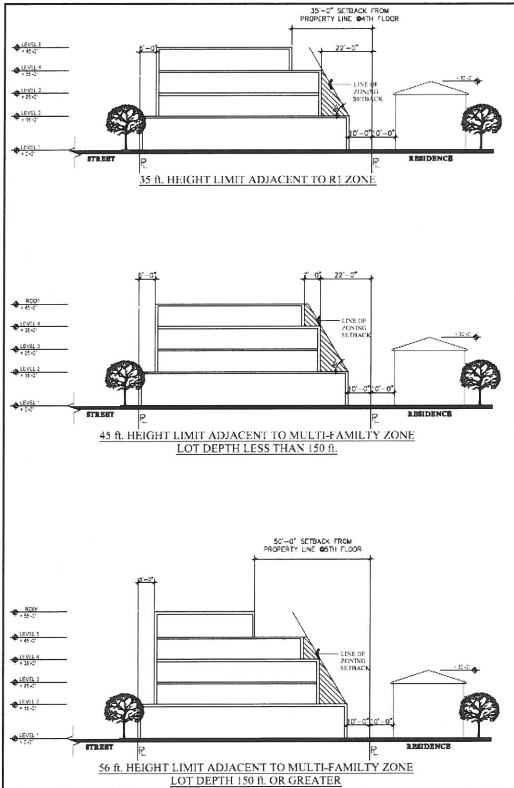
Figure 4-4 Building Height and Setbacks Illustration
