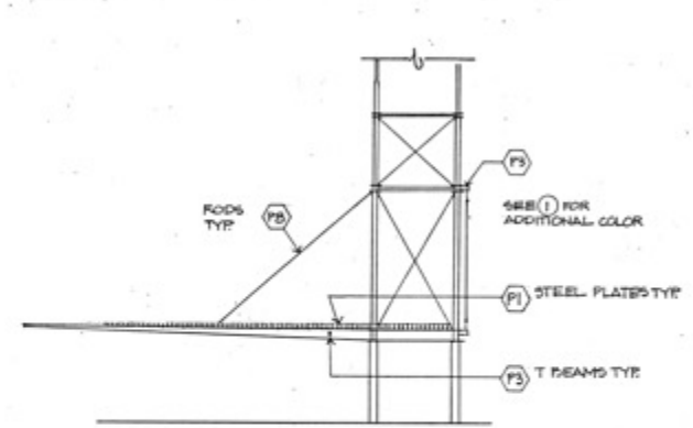
3 ELEVATION SHOWN FOR COLOR ONLY 1/2" = 1'-0"
