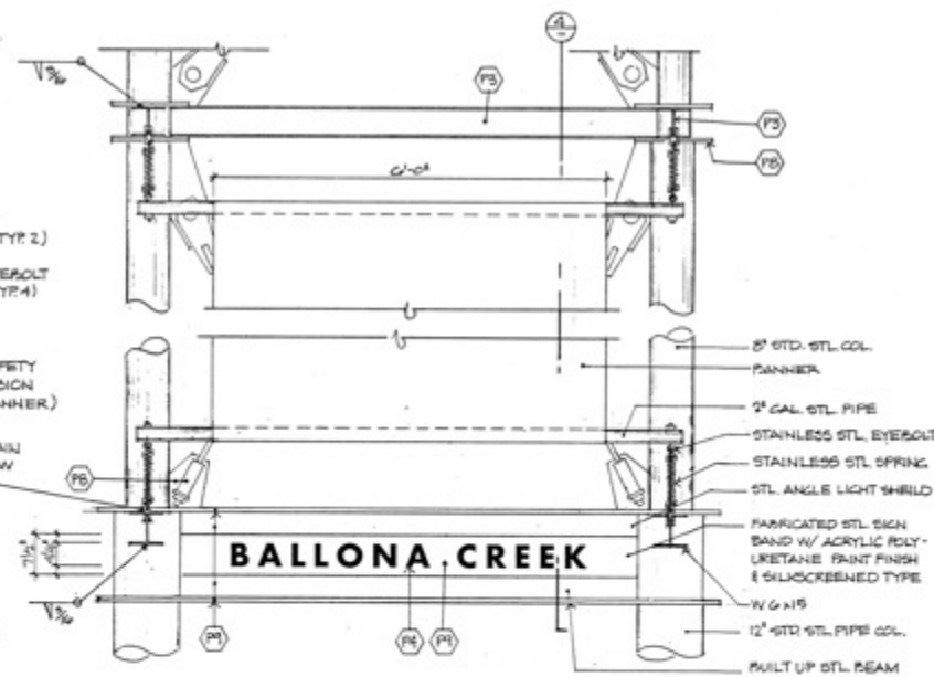
2 DETAIL ELEVATION 1" = 1'-0"
