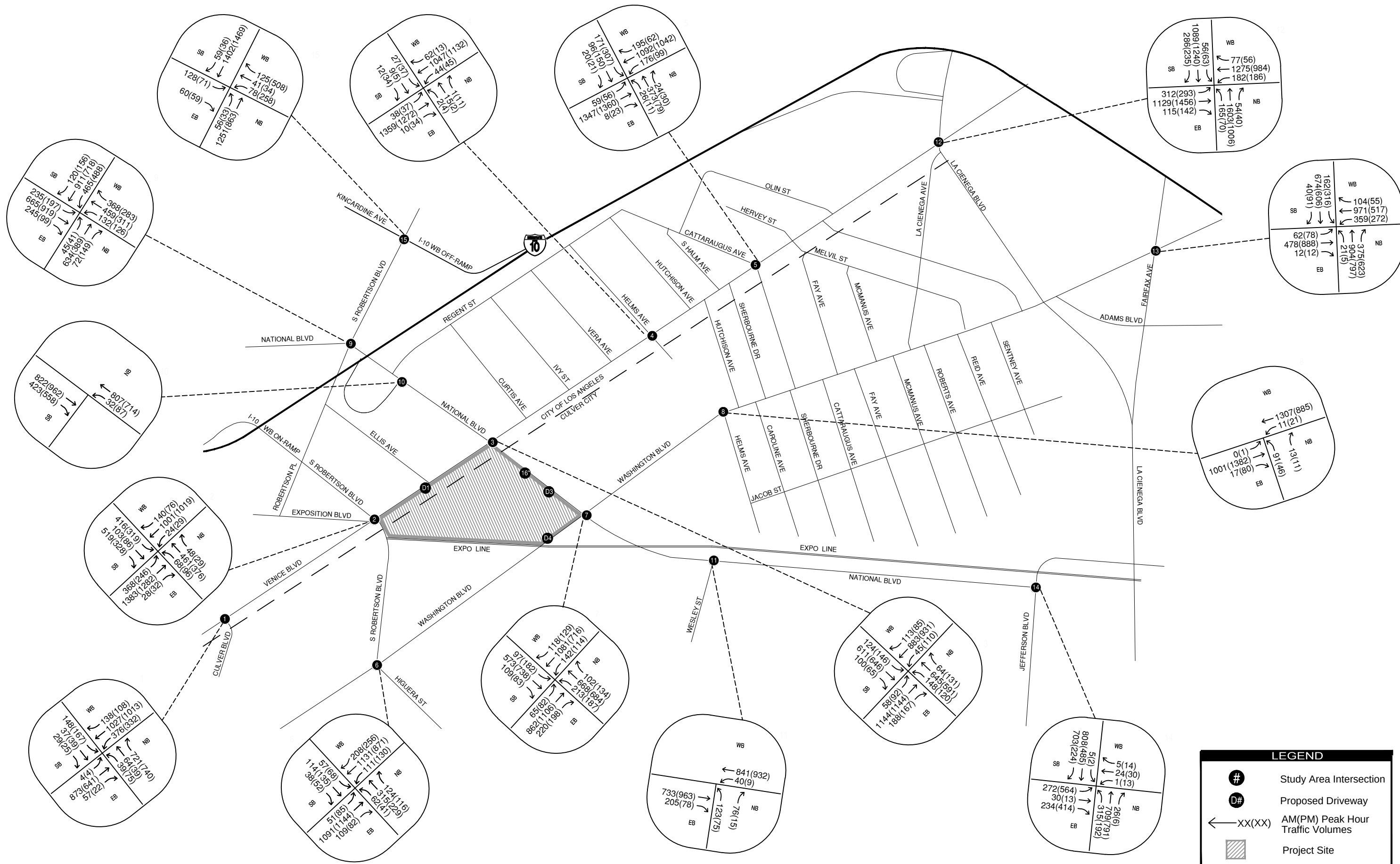
FIGURE 4 - EXISTING (2014) AM(PM) PEAK HOUR TURNING MOVEMENT VOLUMES
