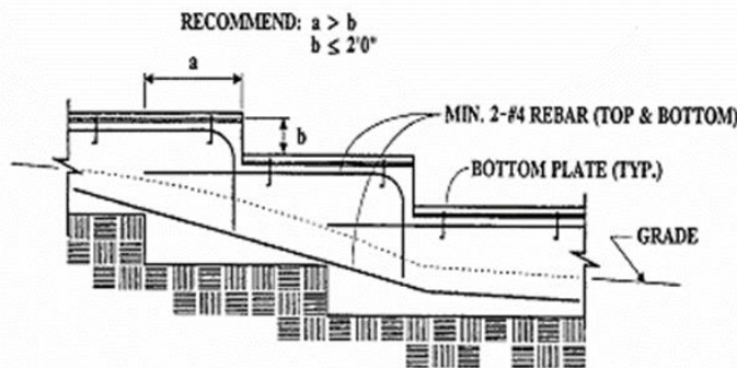
20 21 22 23 24 25 26 STEPPED FOUNDATIONS
