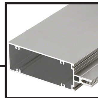
ALUMINUM MULLION, LIGHT GREY
