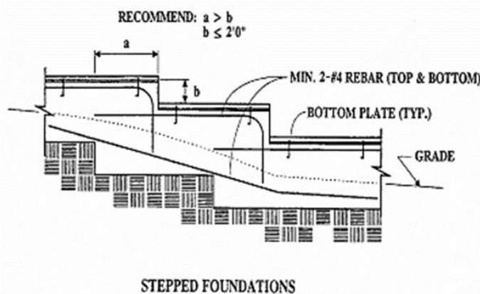
FIGURE R403.1.5 - STEPPED FOOTING
