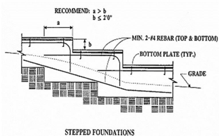
FIGURE 1809.3 - STEPPED FOOTING
