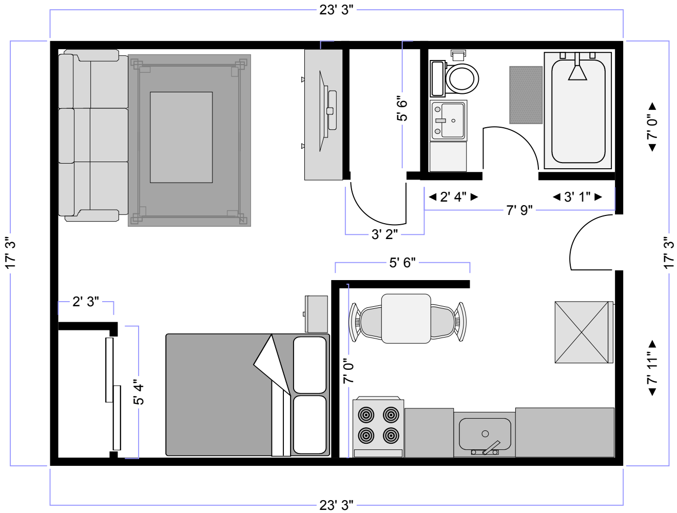
400 Sq. Ft. Floor Plan
