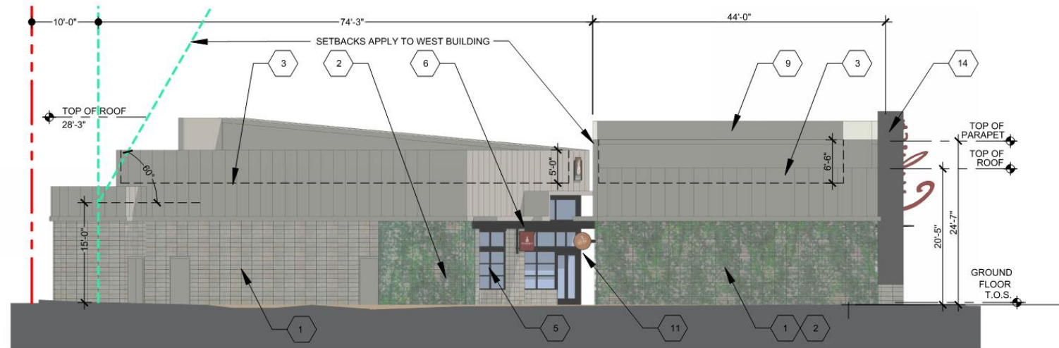
NORTH ELEVATION 03 3/32"=1'-0"
