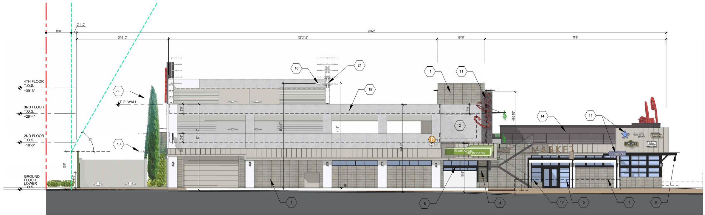
WEST ELEVATION 01 3/32"=1'-0"
