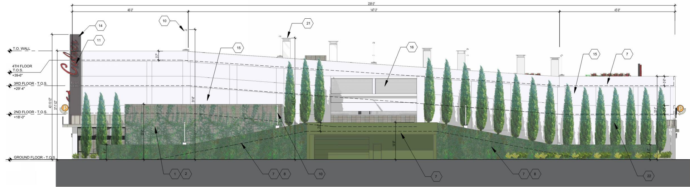
NORTH ELEVATION 02 3/32"=1'-0"
