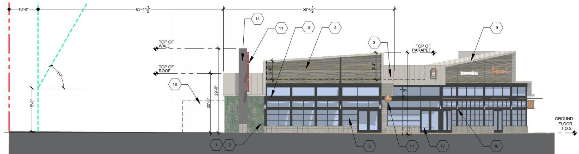
WEST ELEVATION 04 3/32"=1'-0"
