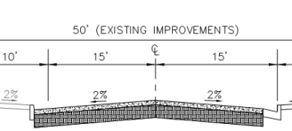
TYPICAL SECTION A-A COLONIAL AVENUE NOT TO SCALE
