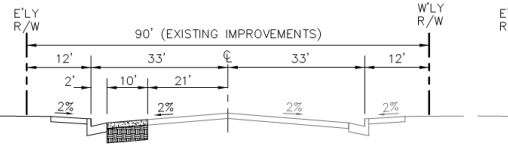
TYPICAL SECTION B-B CENTINELA AVENUE NOT TO SCALE
