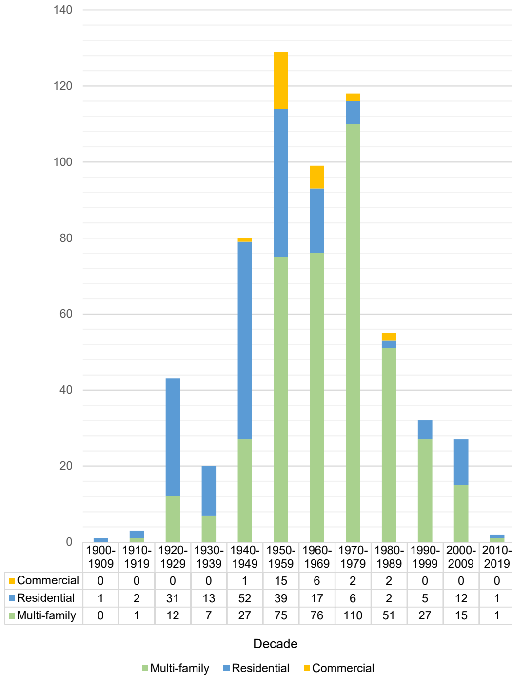
Figure 6 - Number of Potential Wood SWOF Buildings vs. Year of Construction
