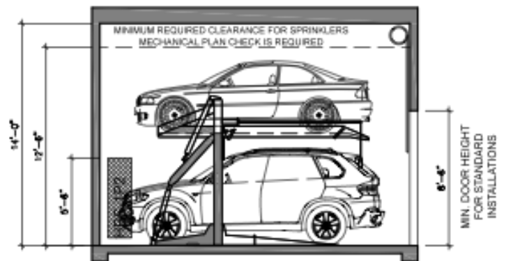
TYPICAL GARAGE SECTION
