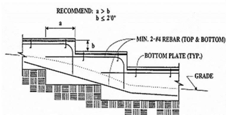
STEPPED FOUNDATIONS
