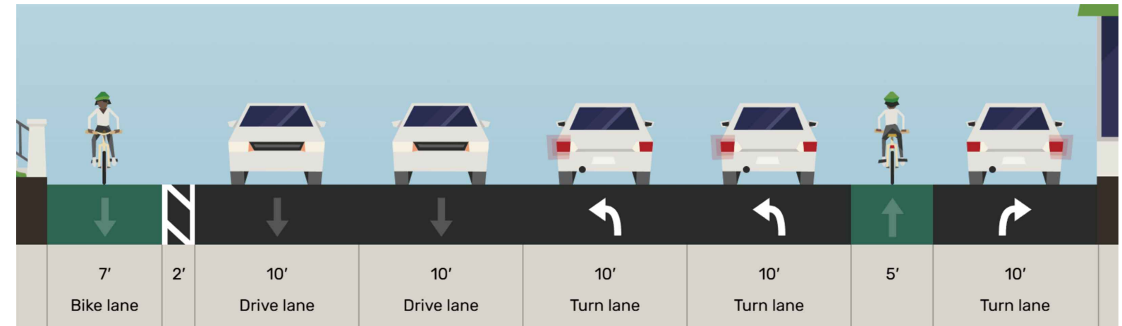
GREEN VALLEY CIR AT SEPULVEDA BLVD PROPOSED STREET CROSS SECTION
