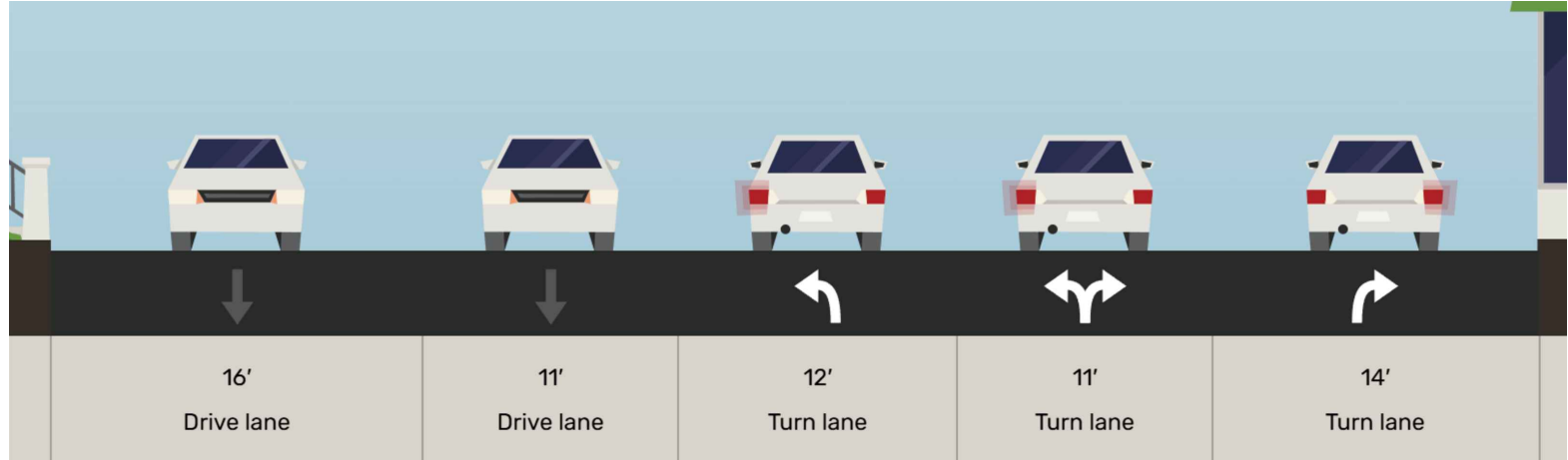
GREEN VALLEY CIR AT SEPULVEDA BLVD EXISTING STREET CROSS SECTION
