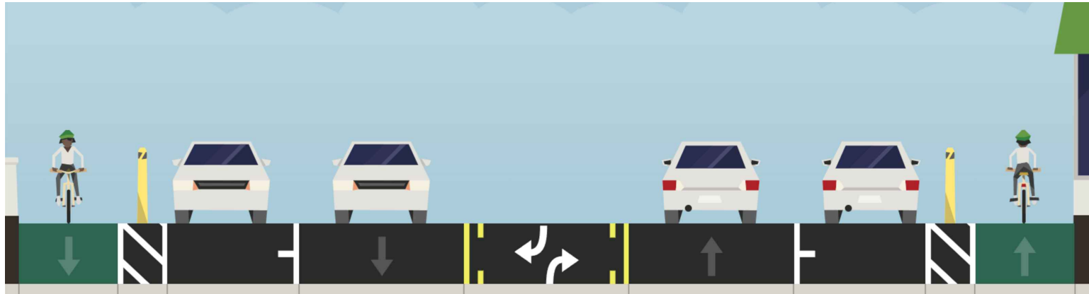
GREEN VALLEY CIRCLE PROPOSED TYPICAL STREET CROSS SECTION
