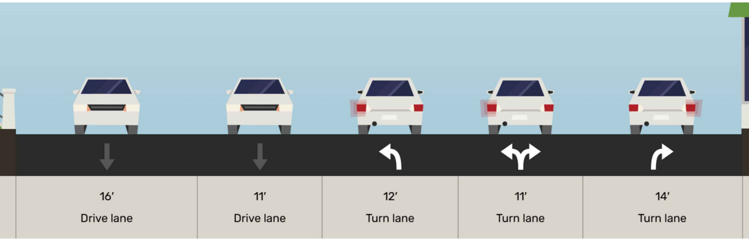
GREEN VALLEY CIRCLE EXISTING TYPICAL STREET CROSS SECTION
