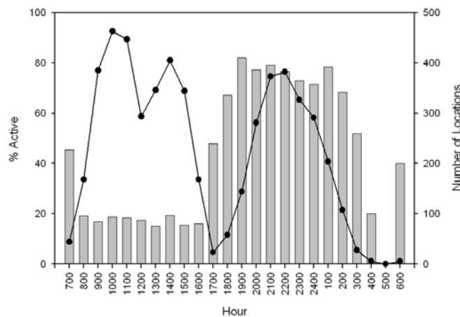
Figure 2. Activity behavior of coyotes in Chicago where bars represent frequency of active locations and lines represent number of locations per hour (Gehrt et al. 2011).
