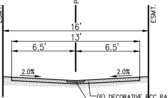
TYPICAL SECTION-PRIVATE STREET
