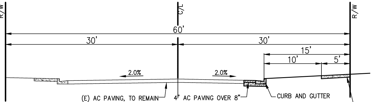
TYPICAL SECTION-LINCOLN AVENUE
