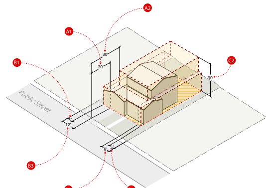
Figure 11 Illustrative Sloped Roof Building at Proposed 0.45 FAR
