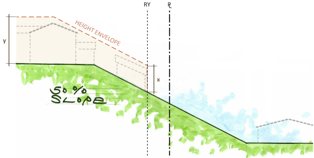
Figure 15 Illustrative diagram of an inclined plane height envelope set from the rear yard setback. The maximum allowable height at the sloped rear yard setback is “x”. The maximum overall allowable height is “y”.
