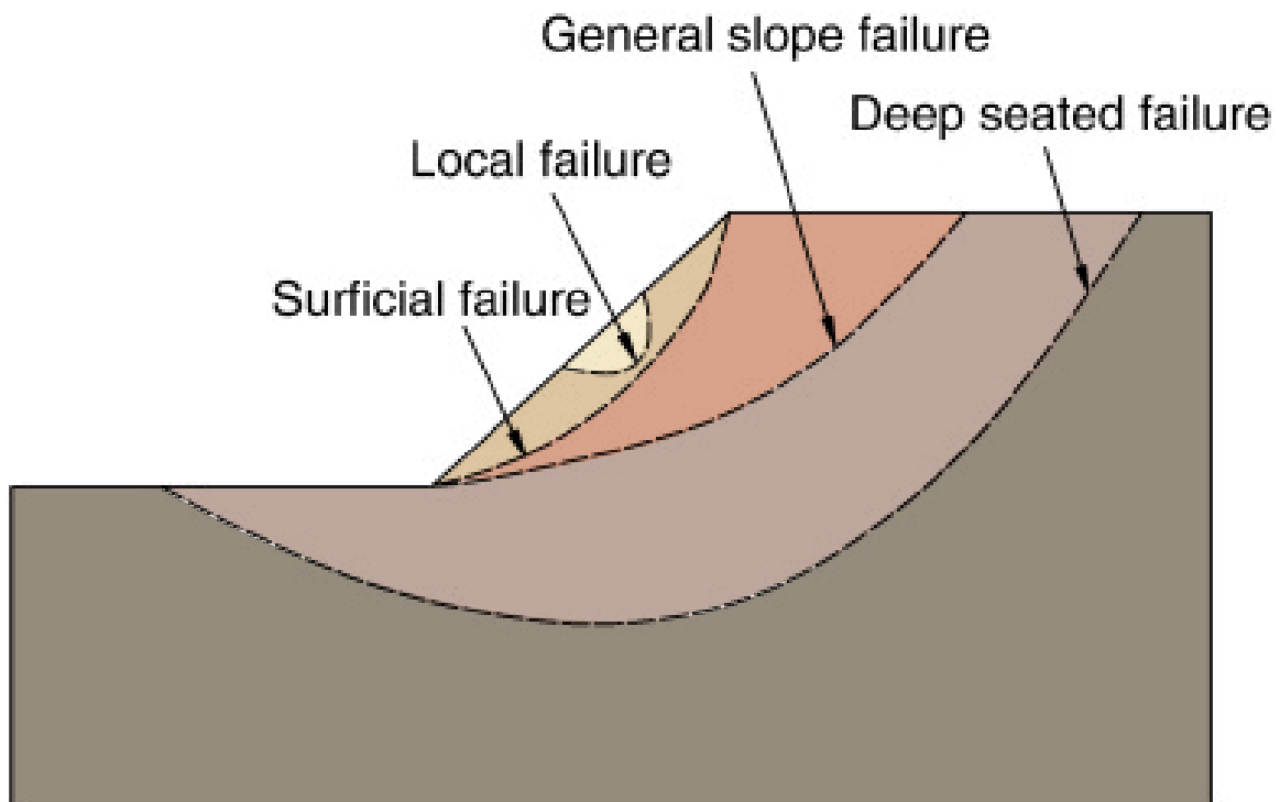
Figure 22 Illustration of Potential Slope Stability Failures. Image from academic paper, "Evaluation of Deep-Seated Slope Stability of Embankments over Deep Mixed Foundations"
