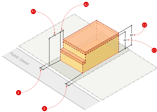
Figure 6 Existing Maximum Zoning Envelope
