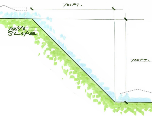
Figure 2 Illustration of Existing and Proposed Slope Thresholds in Culver Crest
