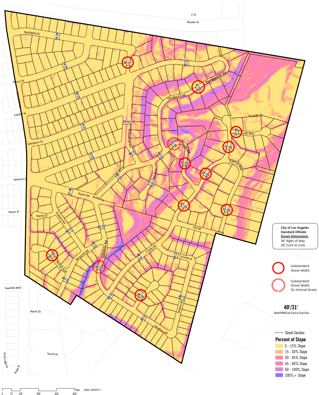
Figure 3 Existing Right-of-Way Map Showing Right-of-Way Constraints
