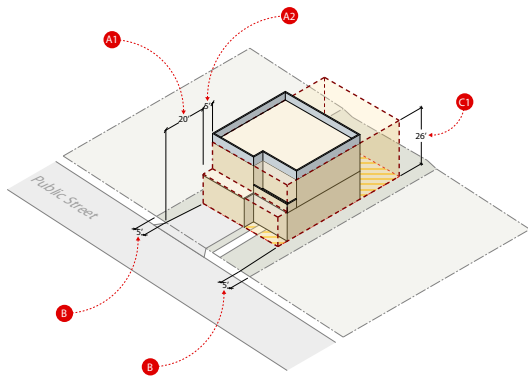
Figure 8 Illustrative Flat Roof Building at Existing 0.6 FAR
