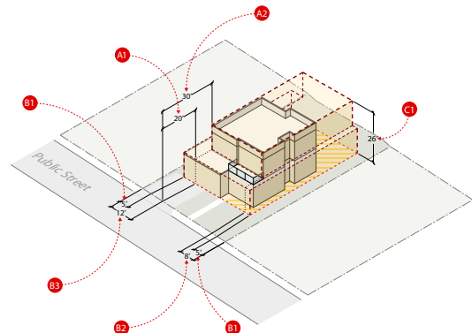
Figure 9 Illustrative Flat Roof Building at Proposed 0.45 FAR
