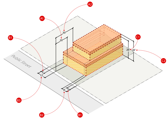
Figure 7 Proposed Maximum Zoning Envelope
