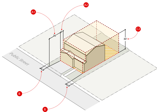
Figure 10 Illustrative Sloped Roof Building at Existing 0.6 FAR
