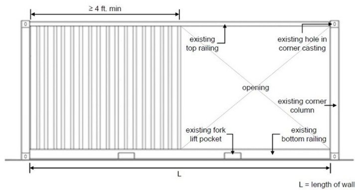
FIGURE 3115.8.5.3(3)~Bracing Unit Distribution—Boundary Elements
