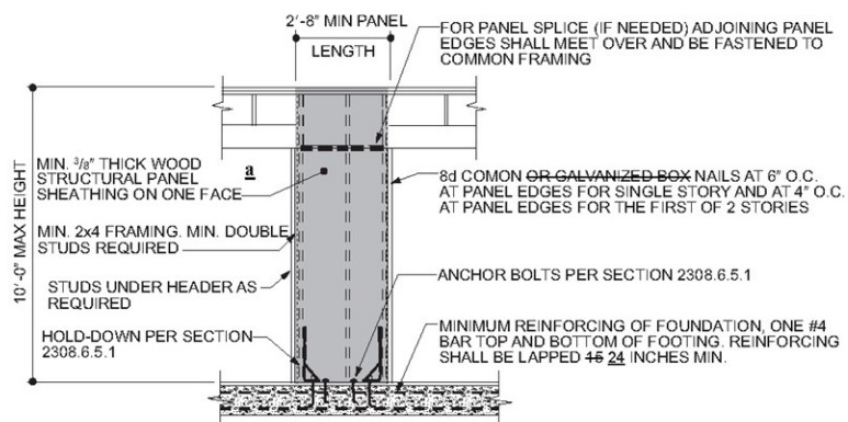
FIGURE 2308.6.5.1 ALTERNATE BRACED WALL PANEL (ABW)
